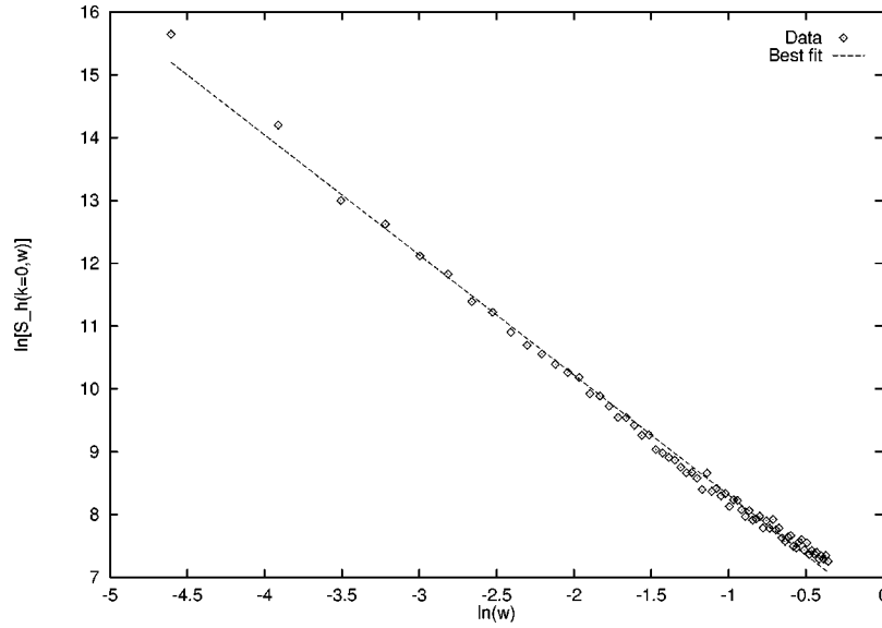
FIG. 11. Log-log plot of the double Fourier transform S_h(k=0, \omega) vs \omega obtained from Eqs. (6) (case B ). The best fit displayed in the figure has a slope of -(1 + 2\beta_h + 1/z_h) = -1.91 \pm 0.017 . Other parameters are \mu = 1.0 , D_h = D_\rho = 1.0 , \Delta_h^2 = \Delta_\rho^2 = 0.5 .
