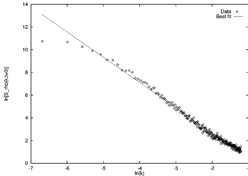
FIG. 12. Log-log plot of the single Fourier transform S_\rho(k, t=0) vs k (case B ) showing a crossover from a slope of -1 - 2\alpha_\rho = 0 at small k to -2.12 \pm 0.017 at large k . Other parameters are \mu = 1.0 , D_h = D_\rho = 1.0 , \Delta_h^2 = \Delta_\rho^2 = 0.5 .
